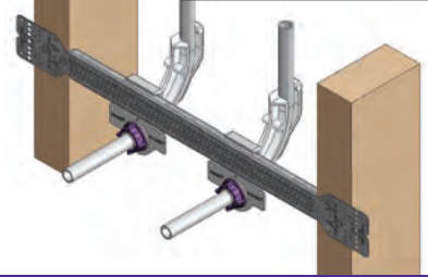
PEX 1/2" Solution Sink
